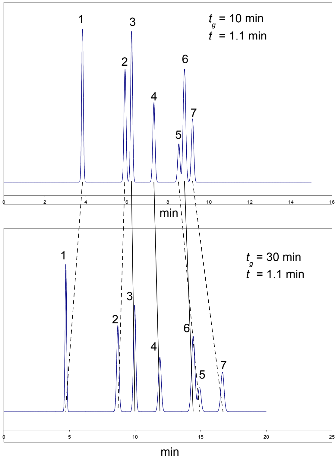
Figure 2: Change in retention with an expansion of the gradient. Top: 10 minute gradient. Bottom: 30 minute gradient. (© Uwe Neue, Waters Corp)
